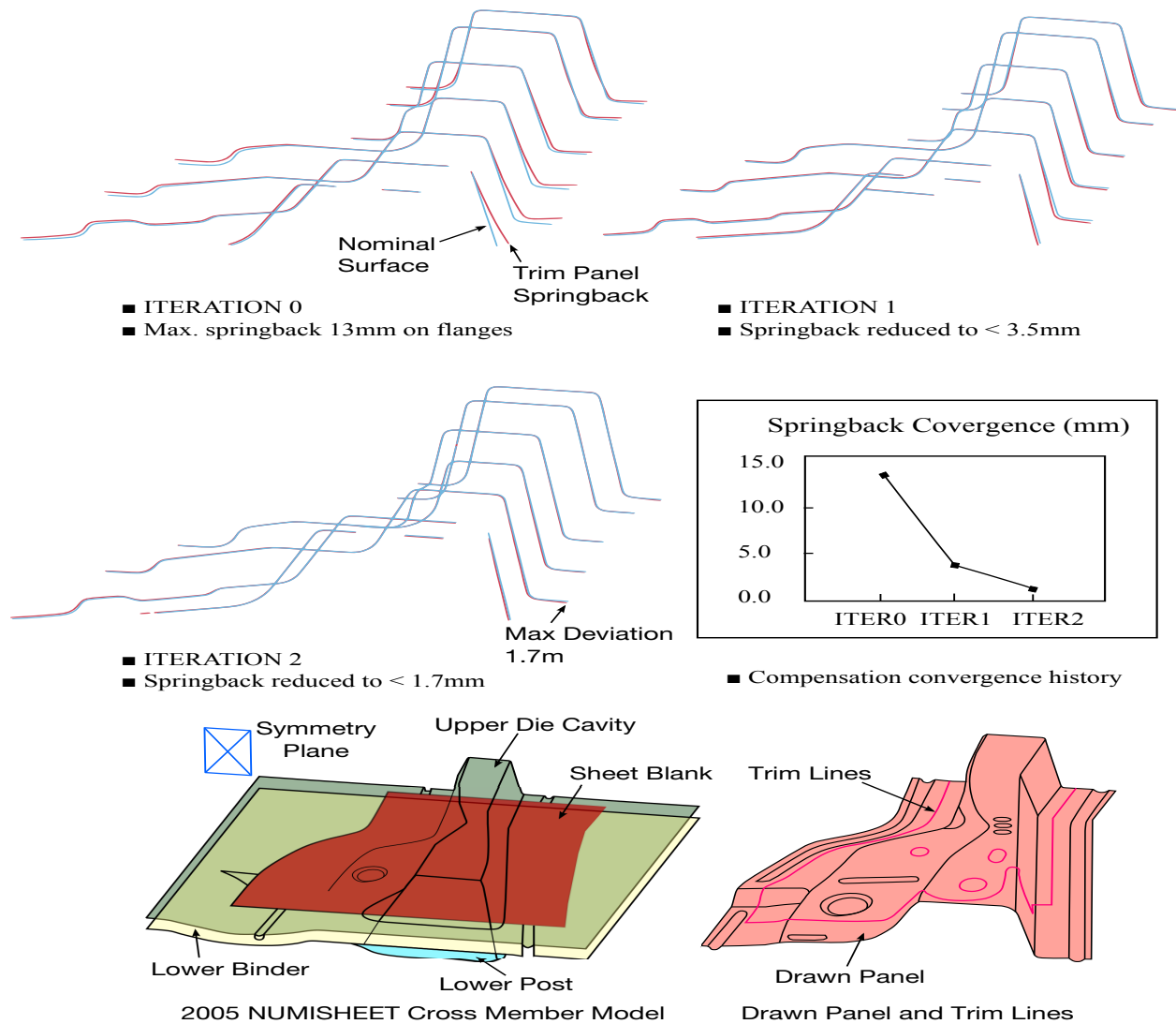
Figure 25-28. Iterative springback compensation on NUMISHEET'05 Xmbr(red – springback, blue – design intent)
