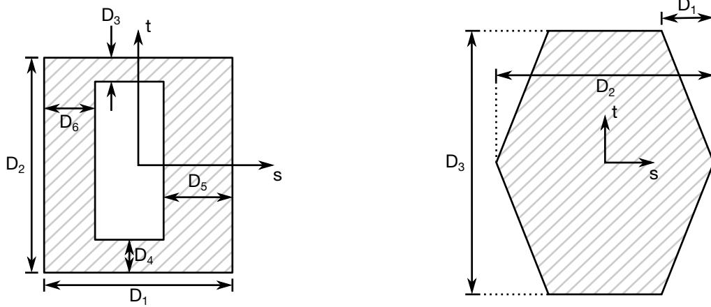
Figure 36-19. SECTION_19 \Rightarrow Box-Shape Figure 36-20. SECTION_20 \Rightarrow Hexagon
