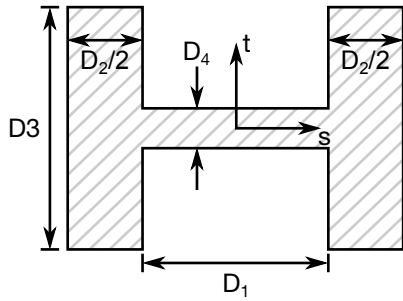
Figure 36-13. SECTION_13 ⇒ H-Shape
