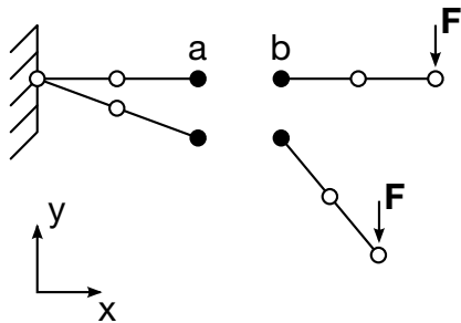
Figure 10-36. Two different ways to constrain node a and b . For rigid-body type situations this card, *CONSTRAINED_NODE_SET may lead to unphysical results.
