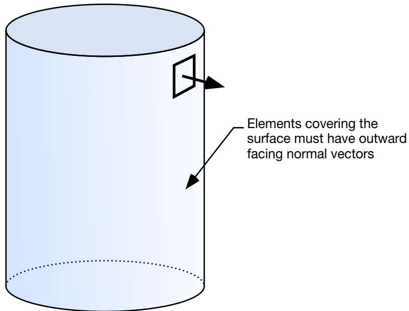
Figure 27-6. The shell elements interacting with the fluid must be numbered such that their outward normal vector points into the fluid media.
