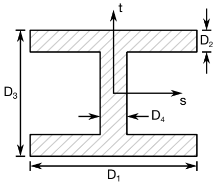
Figure 36-1. SECTION_01 ⇒ I-Shape
