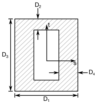
Figure 36-5. SECTION_05 ⇒ Box-Shape
