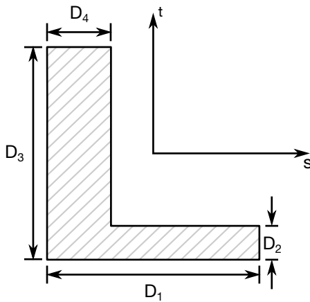
Figure 36-3. SECTION_03 ⇒ L-Shape
