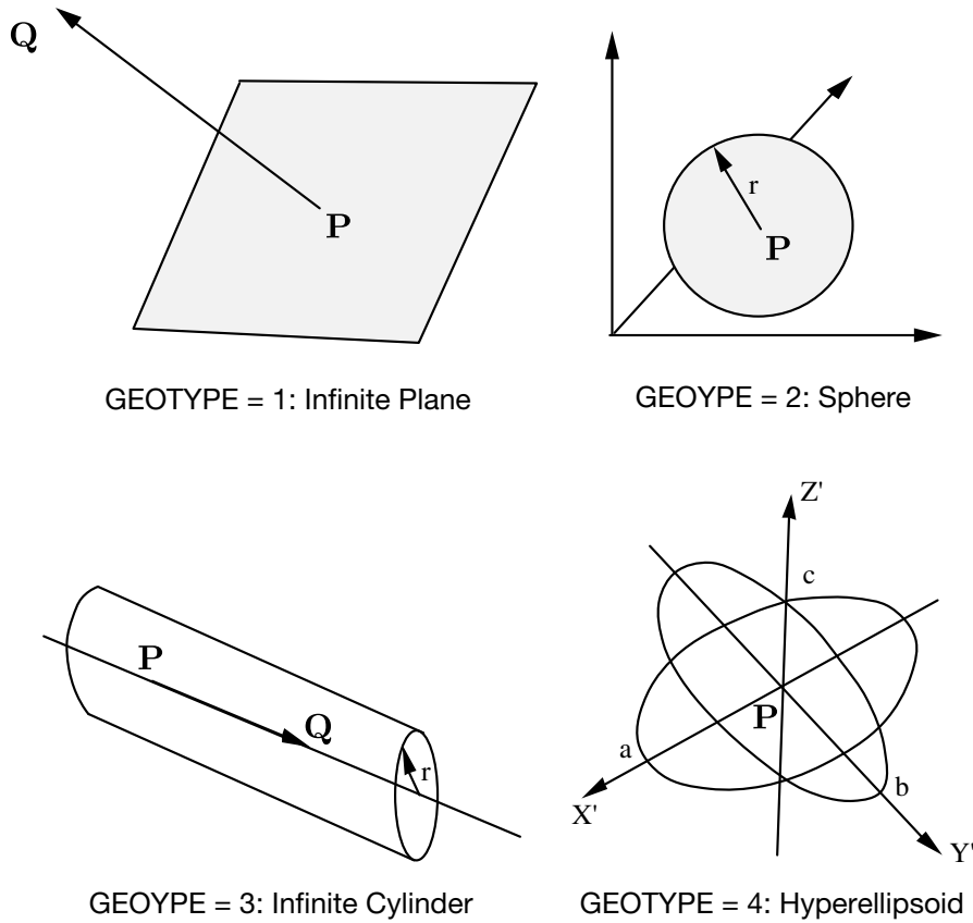
Figure 11-24. Contact Entities.
