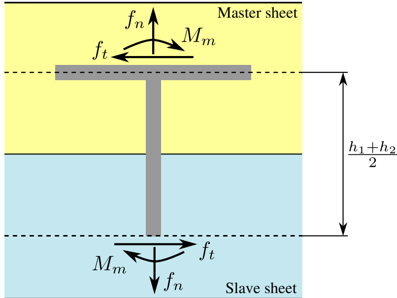
Figure 10-42. Local forces/moments.
