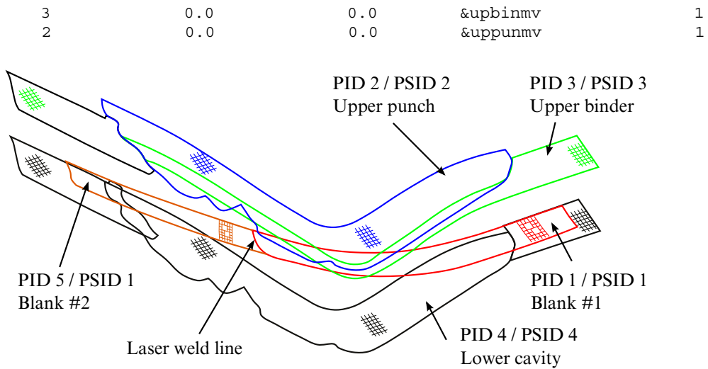
Figure 31-1. A tailor welded blank is positioned in a decklid (toggle draw).
