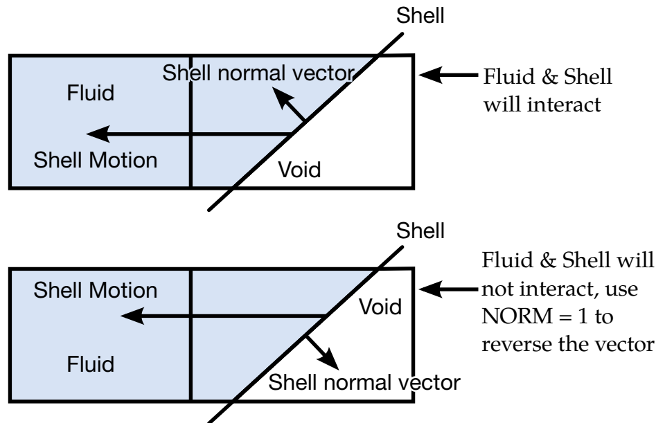
Figure 10-32. Shell Motion
