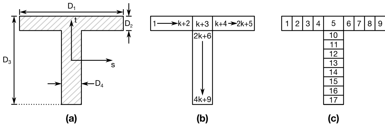
Figure 24-6. Type 4: T-shape. (a) Cross section geometry. (b) Integration point numbering. (c) Example for k = 2 .
