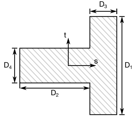
Figure 36-14. SECTION_14 ⇒ T-Shape 2
