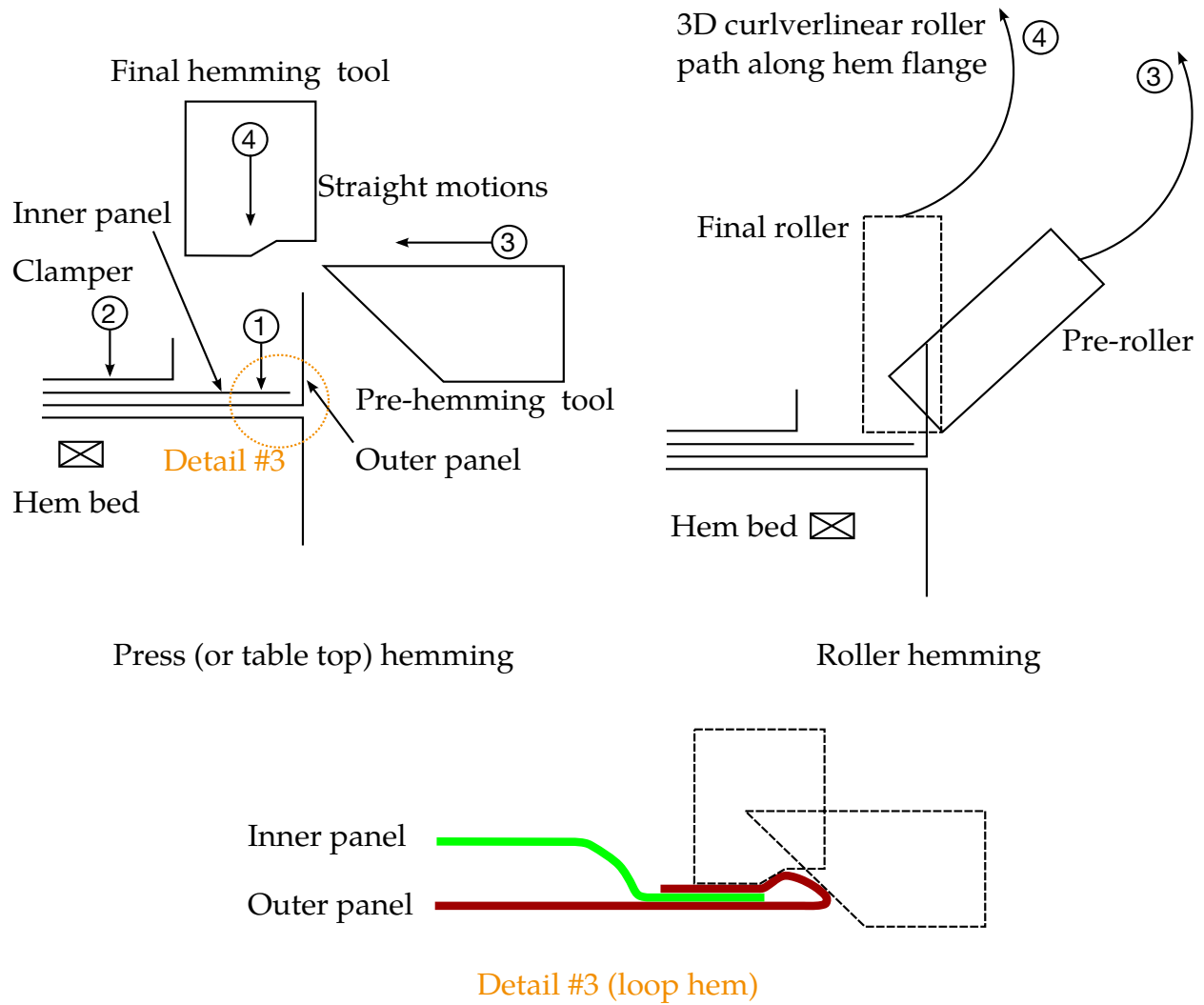
Figure 63-4. Types of hemming dies
