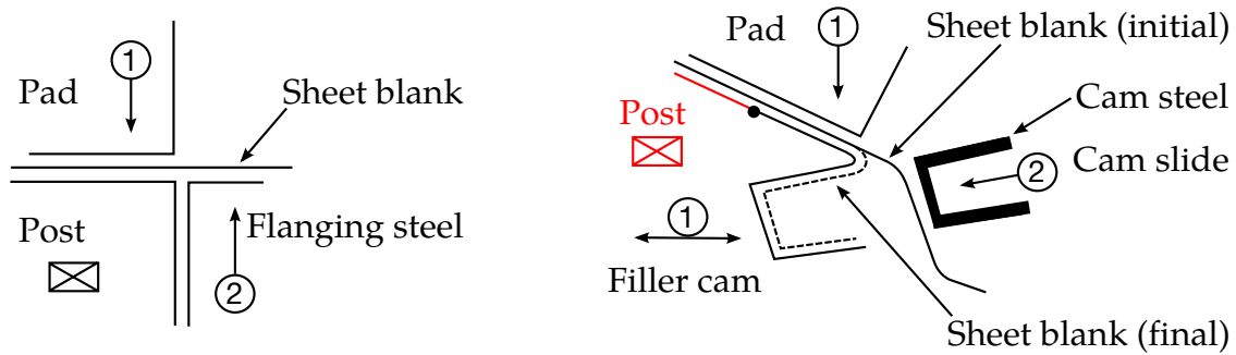
Direct flanging
