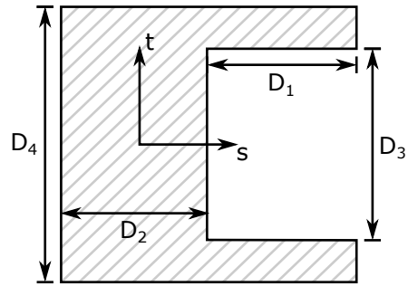
Figure 36-16. SECTION_16 ⇒ Channel 2
