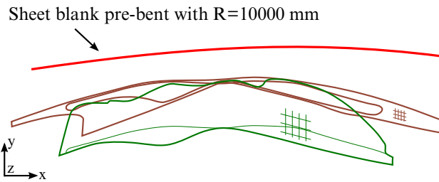
Figure 12-41. Pre-bending using this keyword (1 st state of D3plots).
