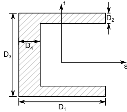
Figure 36-2. SECTION_02 ⇒ Channel
