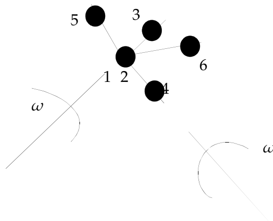
Figure 10-25. Constant velocity joint. Nodal pairs (1, 3) and (2, 4) define axes for the constant angular velocity, and nodal pairs (1, 5) are orthogonal vectors. Here nodal points 1 and 2 must be coincident.
